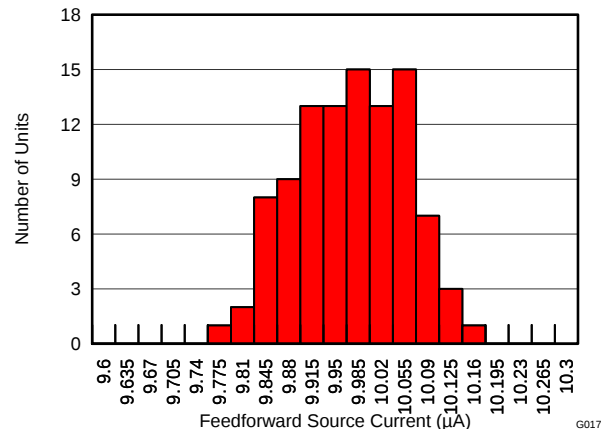
Figure 16. Feedforward Source Current ( I_{\text{FF}} ) Variation ( I_{\text{VAC}}=100\text{ }\mu\text{A} , Temperature = 25^{\circ}\text{C} )
