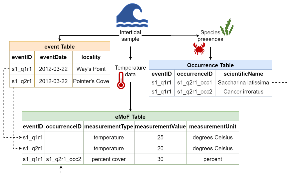
Figure 14.2: Example of how sample data is distributed to core and extension tables, and how these tables are connected in OBIS
