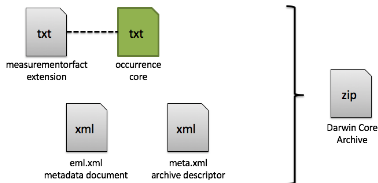
Figure 37.1: Example showing how Occurrence core, EML, and meta.xml files make up a Darwin Core-Archive file
