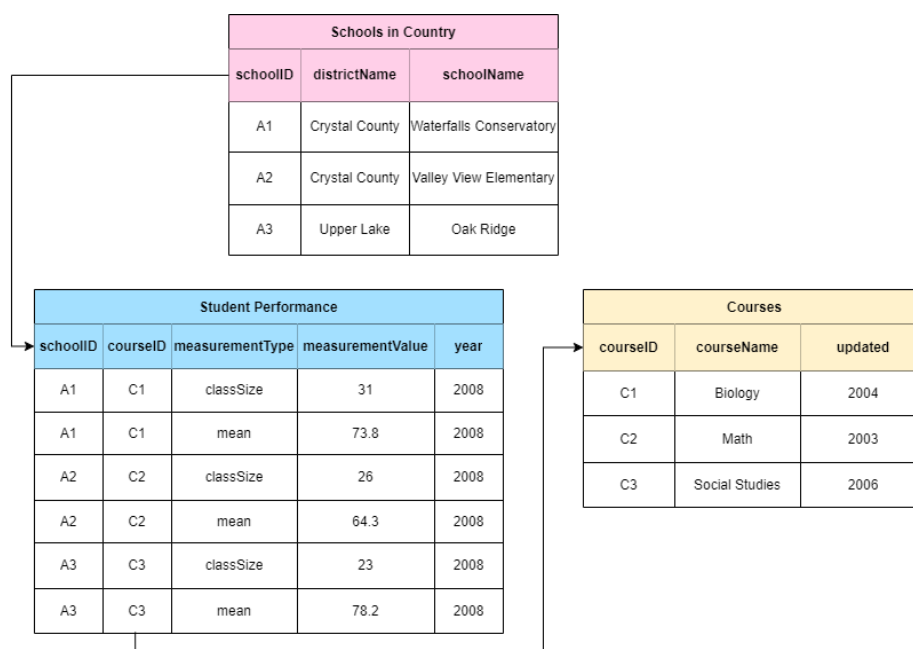
Figure 14.1: An example of how a relational database works. Three tables show the (1) student performance (blue table) in (2) different schools (pink table) in a fictional country, and (3) the names of the courses (yellow table). Information between each table is linked by the use of identifiers, indicated by the arrows
