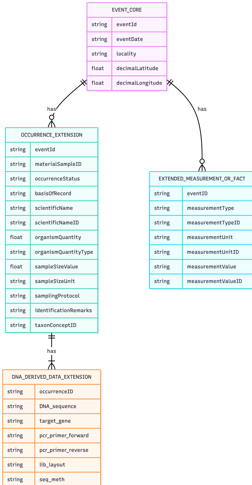
Figure 25.3: Show general structure of a DNA dataset using the event core and occurrence extension tables
