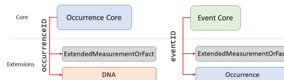
Figure 17.2: Diagram of how the different core tables are linked to their extensions by different identifiers.
