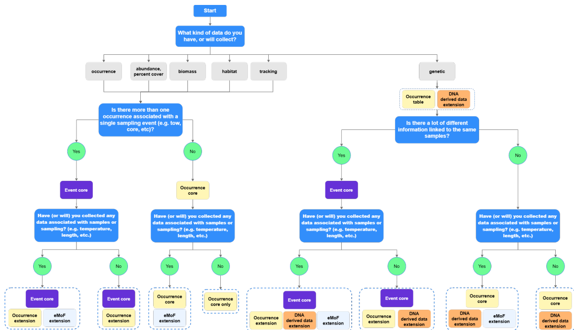
Figure 17.1: Flow chart to help determine which dataset structure will suit your data
